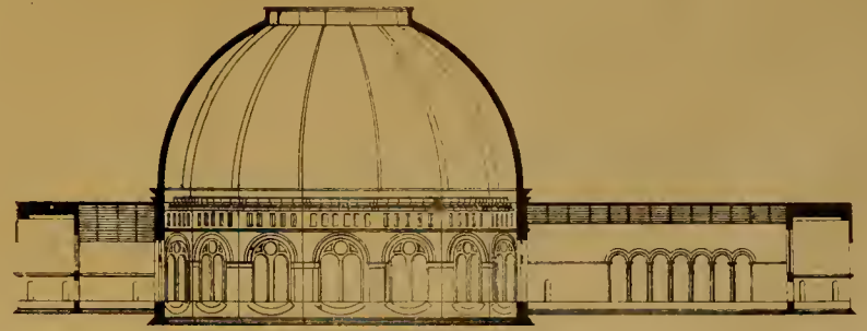
SECTION THROUGH CENTRE HALL ON THE LINE A B.
