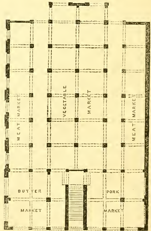
PLAN OF MARKET.
