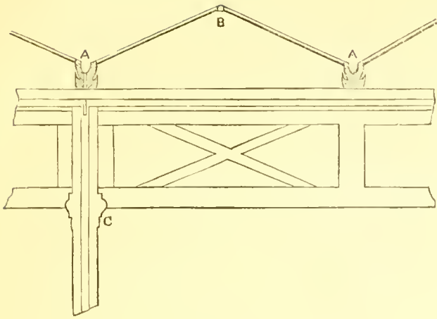
Fig. 6.—Transverse View of Ridge-and-Furrow Skylight.
