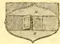
Fig. 11.—B, Water-tight Bulkheads, Sections at end of Midship Sections, showing the sections as a Deck-house.
