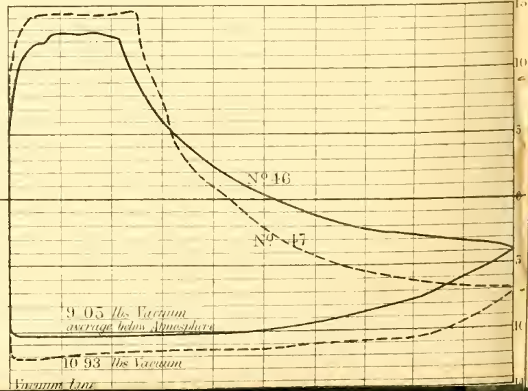
Fig 5 Diagram from pair of Blast Engines
