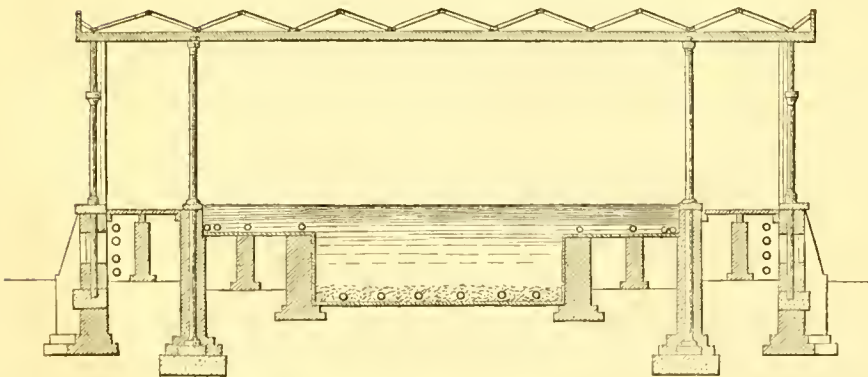
Fig. 2.—Transverse Section.
