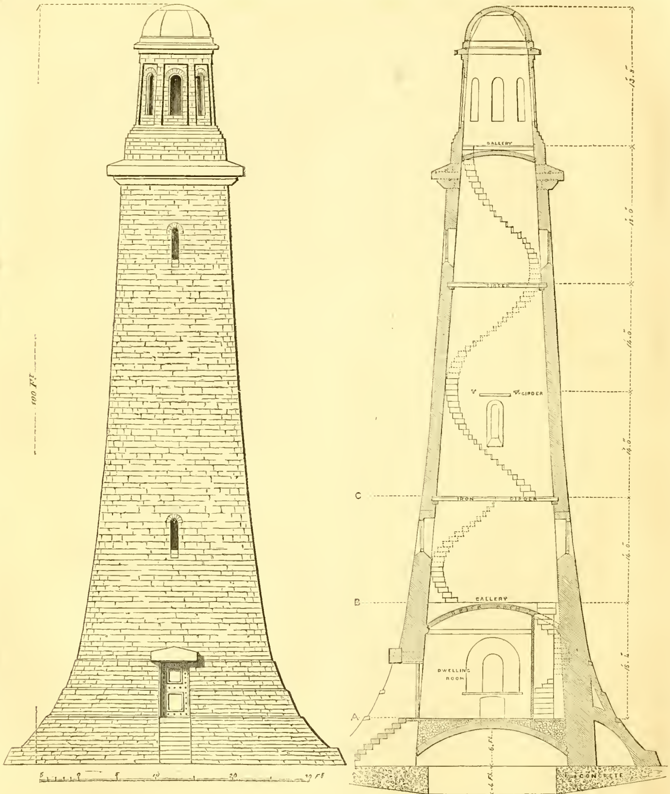
ELEVATION.
