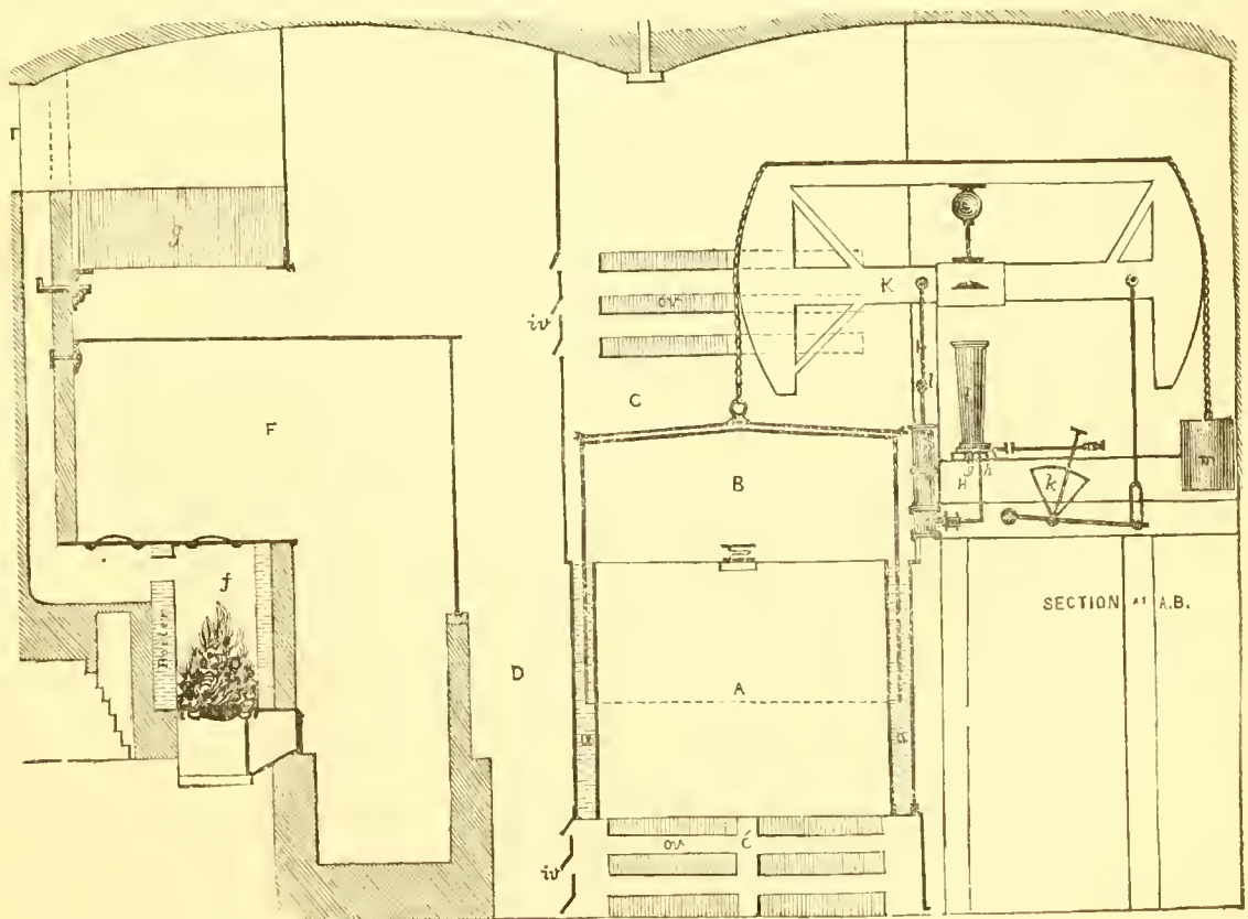
Fig. 2.—SECTION.
