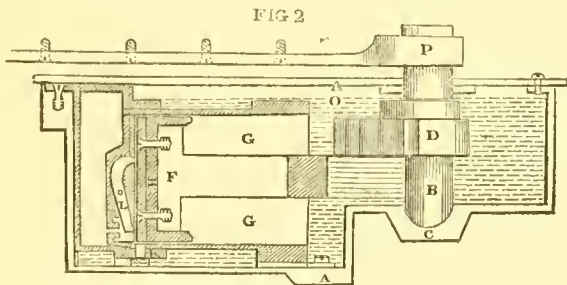
FIG 2. VERTICAL SECTION.
