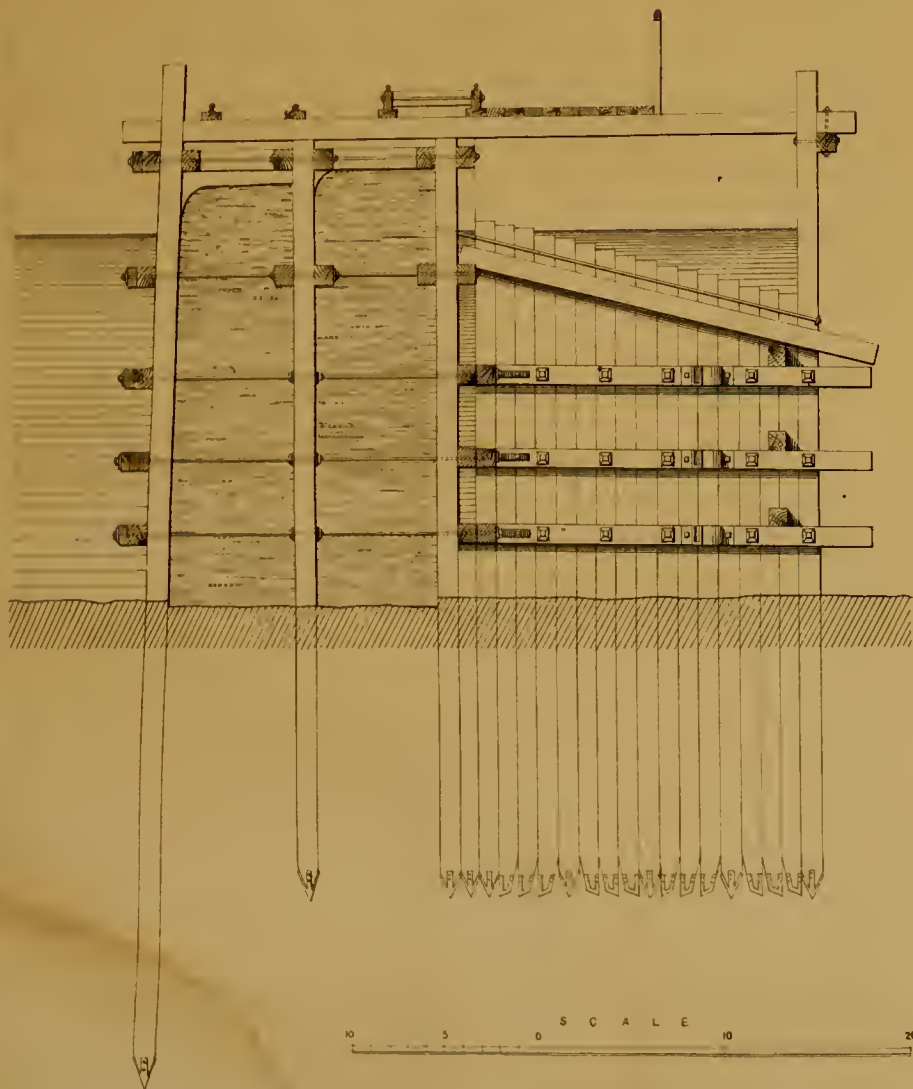
TRANSVERSE SECTION.
