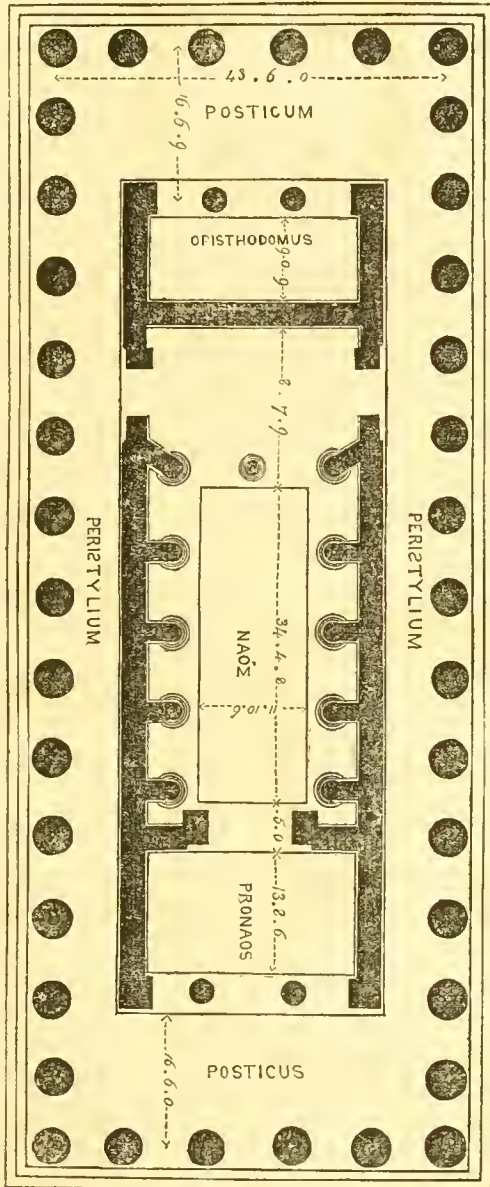
Peripteral Temple of Apollo Epicurius, at Bassæ.
